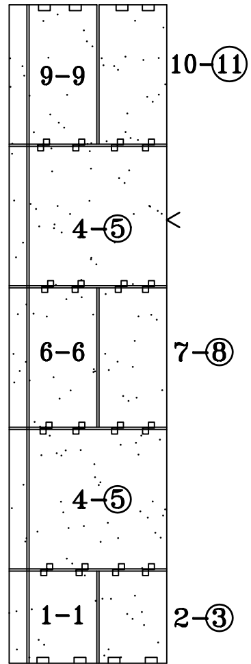
1 STONE VENEER ELEVATION 1 THUS/1 OH
