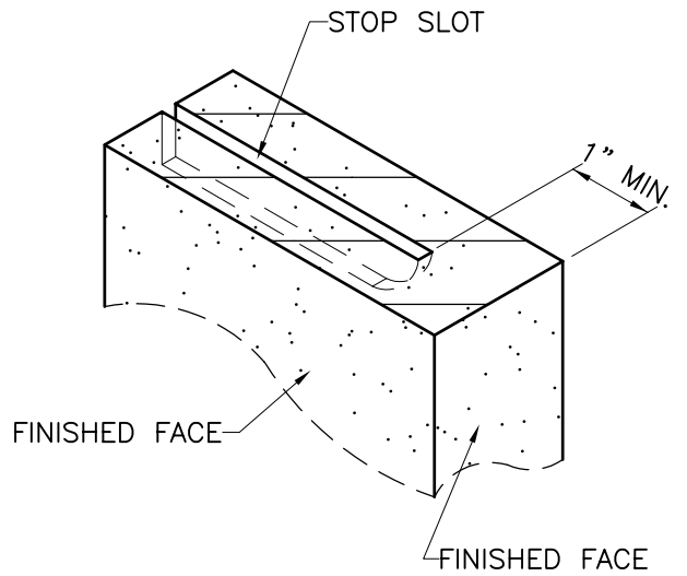
STOP ANCHOR SLOT
