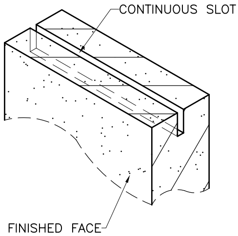
CONTINUOUS ANCHOR SLOT
